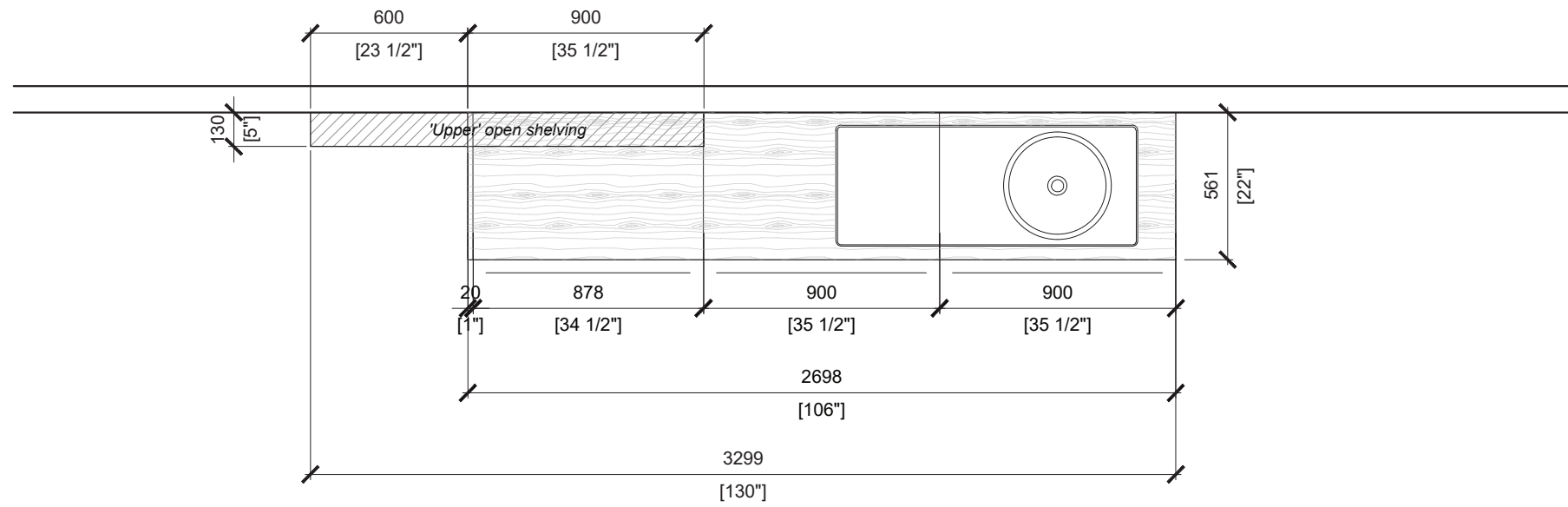
PARTIAL PLAN
