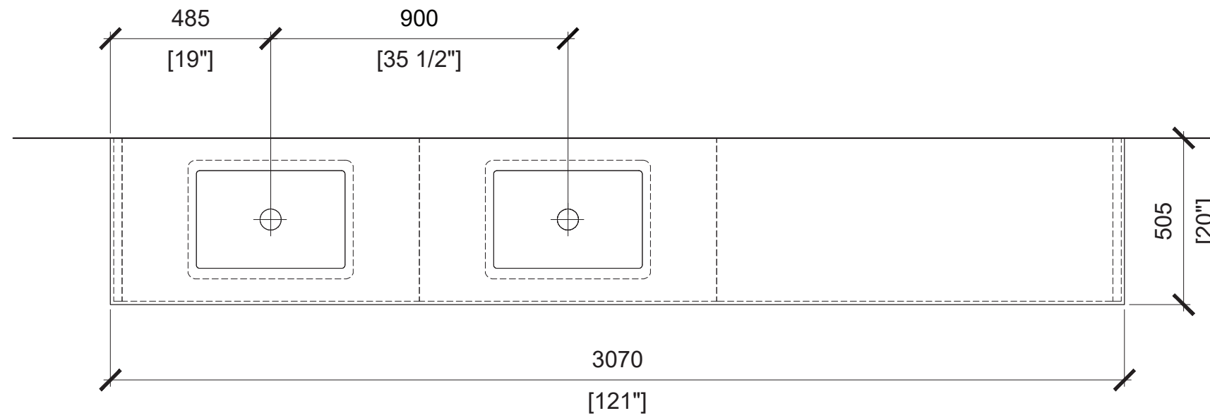
PARTIAL PLAN
